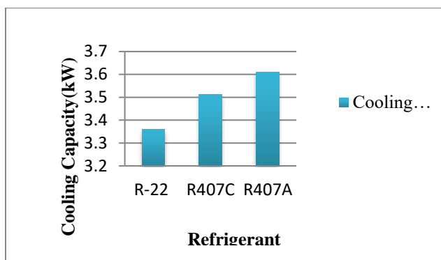
Fig.4. cooling capacity comparison of the refrigerants
