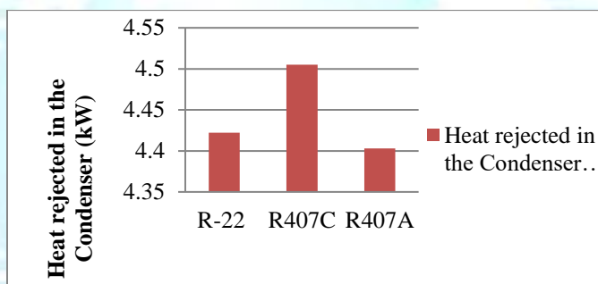
Fig.5. Comparison of heat rejected in the condenser
