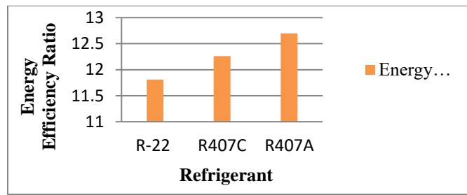
Fig.7. Energy Efficiency Ratio comparison of the refrigerants
