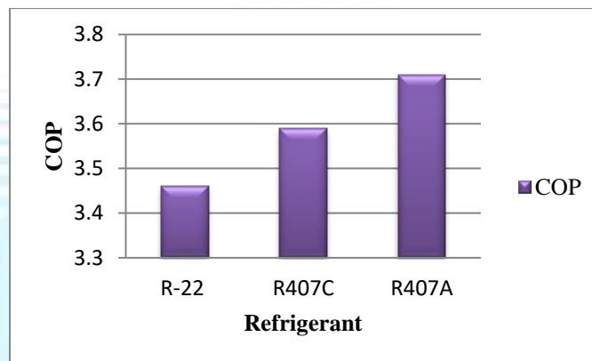
Fig.8. COP comparison of the refrigerants
